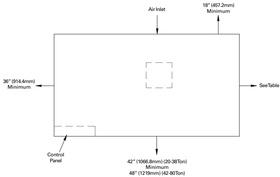
Top View SCWF/SCRF/SIWF/SIRF
